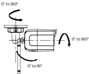
Figure 3-5 View Angle Adjustment
