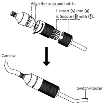
Figure 3-7 Waterproof Accessory Installation
