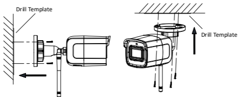
Figure 3-4 Install the Camera
