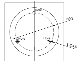
Figure 3-3 Drill the Holes
