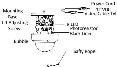
Figure 1-3 Overview of Type III Camera
