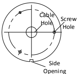
Figure 2-2 Drill Template
