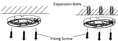
Figure 2-12 Fix the Mounting Base to the Ceiling
