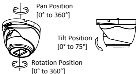
Figure 2-11 3-axis Adjustment
