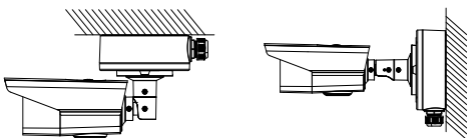
Figure 2-6 Fix the Junction Box Cover back to its Body
