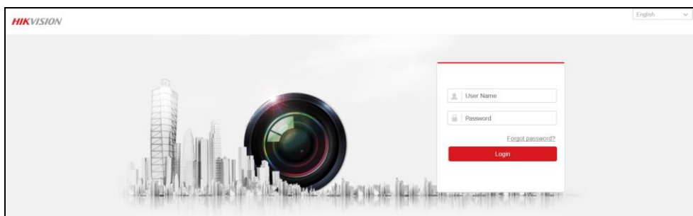
Figure 4. 1 Login Page
