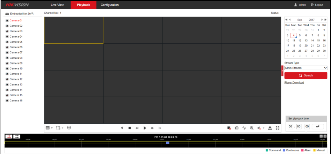
Figure 4. 6 Playback
