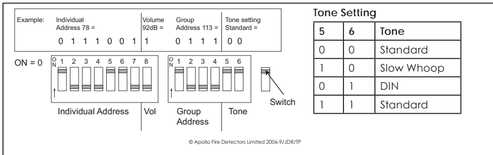
Fig 3. Example of address and tone setting
