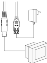
Figure 2-17 The Power/Video Cable (Two-pins Power Interface)
