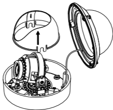
Figure 2-2 Remove the Black Liner
